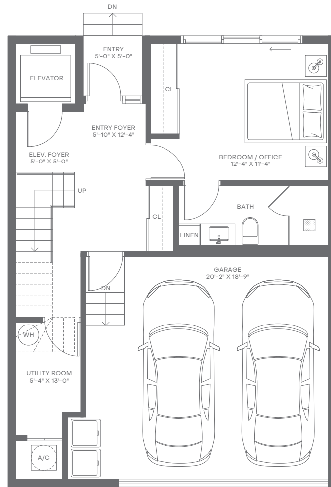
LEVEL 1
