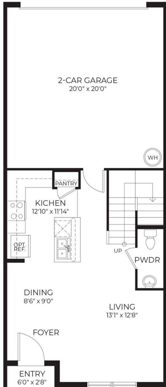
FIRST FLOOR
