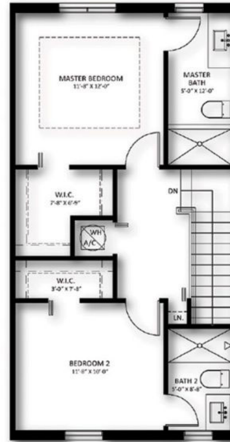
SECOND FLOOR
