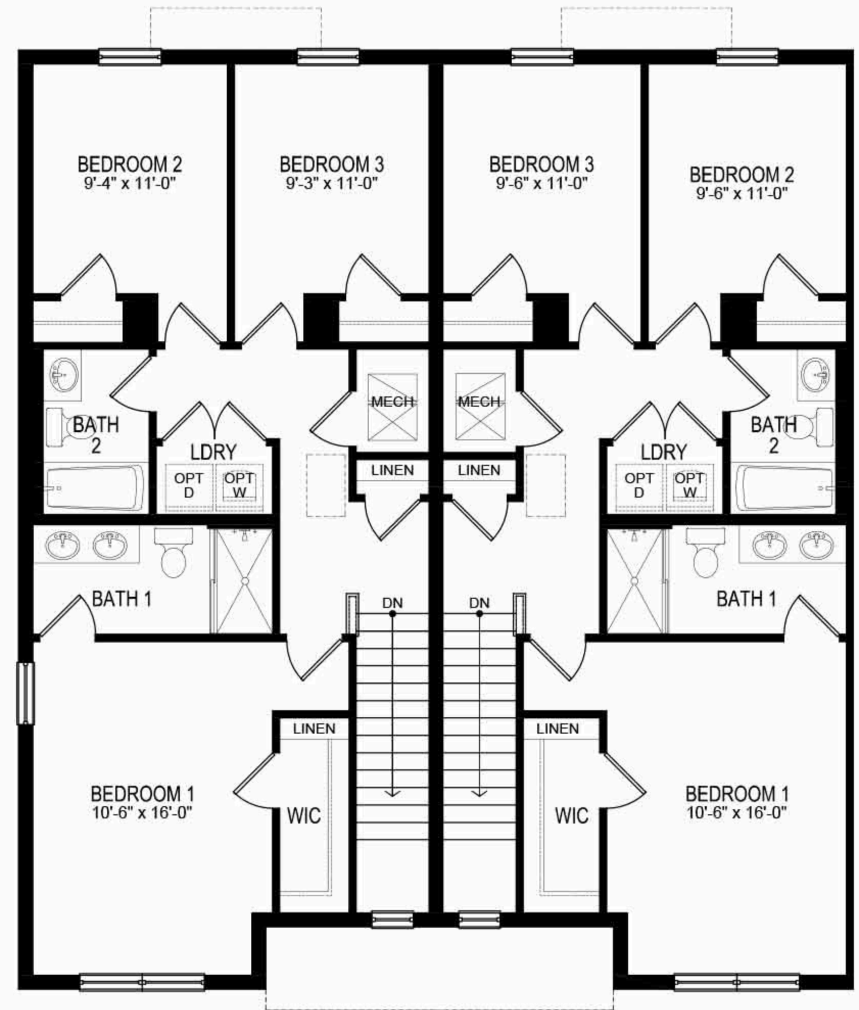
SECOND FLOOR
