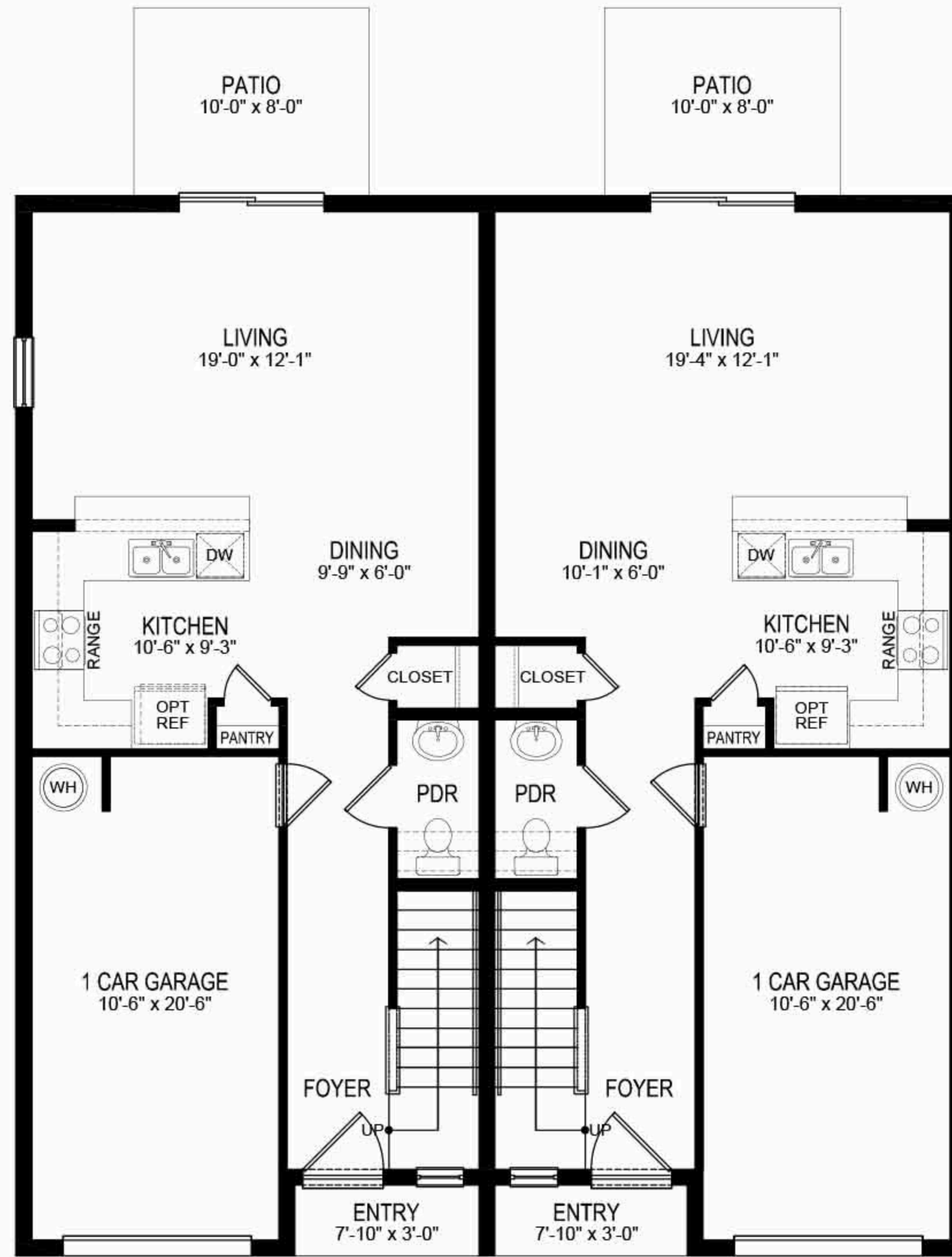
FIRST FLOOR
