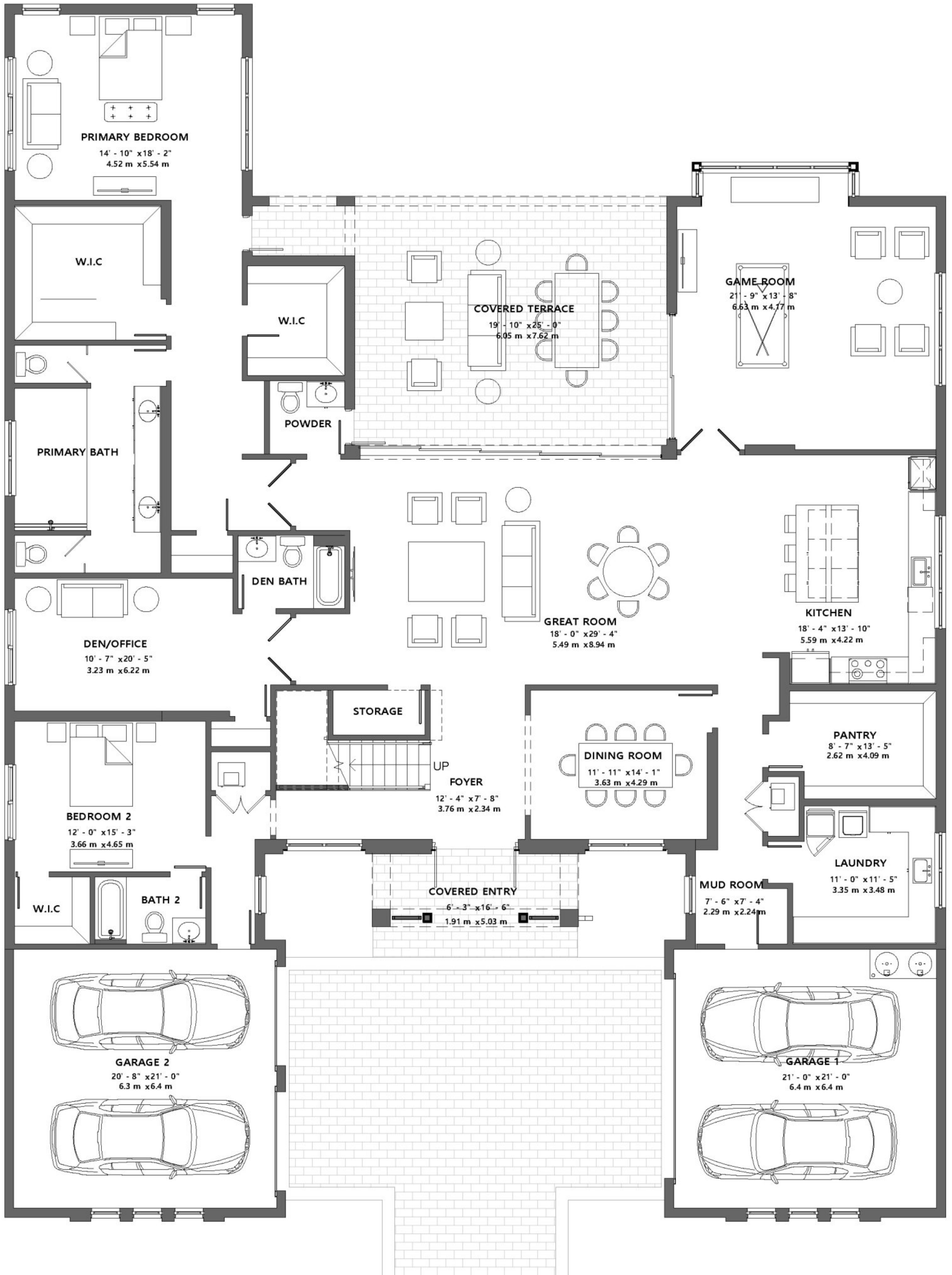
FIRST FLOOR STANDARD PLAN
