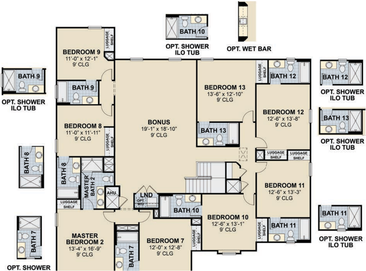
SECOND FLOOR A
