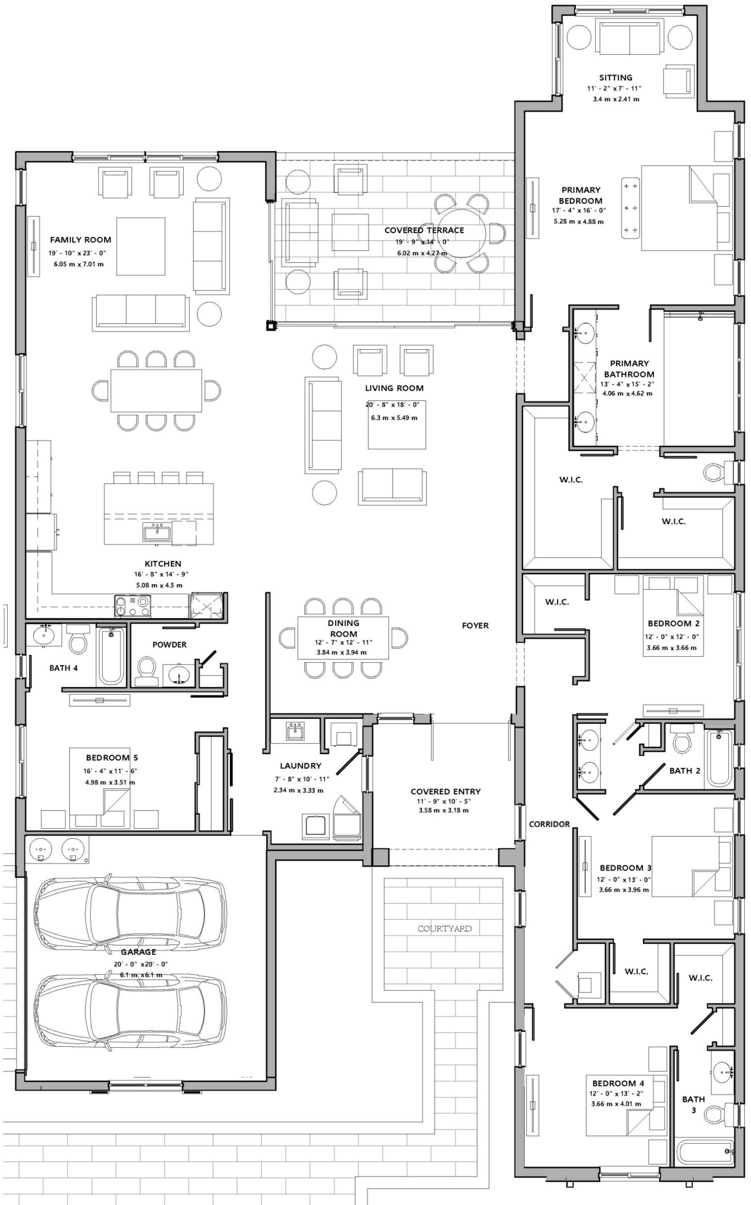
FIRST FLOOR STANDARD
